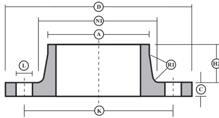
Steel Welding Neck Flange
