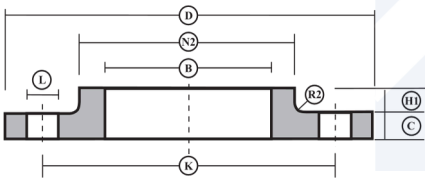
Slip-on Boss Flange
