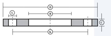
Steel Plate Slip-on Flange
